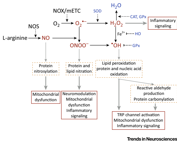
Figure 1. Induction of Nitroxidative Species after Tissue Injury. Nitroxidative species can induce post-translational modifications of proteins and lipids, which subsequently drive pathological pain by modulating nociceptive neurotransmission, activating TRP channels, and inducing mitochondrial dysfunction, and thereby induce inflammatory signaling. In healthy cells, endogenous antioxidant systems prevent nitroxidative damage. Cell damage/pathology can perturb this balance, driving the accumulation of potentially damaging nitroxidative species. Abbreviations: CAT, catalase; GPx, glutathione; H_2O_2 , hydrogen peroxide; HO, heme oxygenase; mETC, mitochondrial electron transport chain; NO, nitric oxide; NOS, nitric oxide synthase; NOX, NADPH oxidase; O_2^{\bullet-} , superoxide; \bullet OH , hydroxyl radical; ONOO^- , peroxynitrite; SOD, superoxide dismutase.
