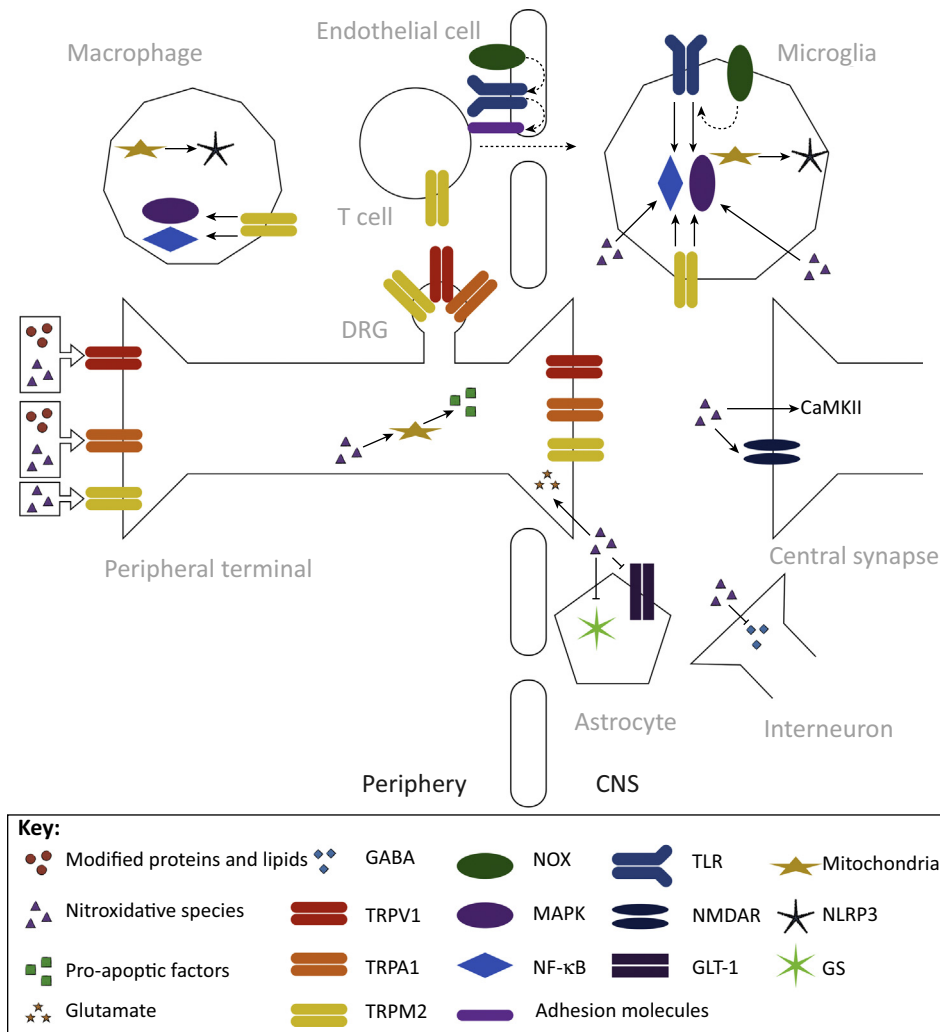
Figure 3. Nitroxidative Mechanisms of Neuroexcitability after Tissue Injury. Reactive nitroxidative species, such as hydrogen peroxide and peroxynitrite, and modified proteins and lipids, including carbonylated proteins, peroxidated and nitrated lipids, and reactive aldehydes, all contribute to peripheral and central sensitization after tissue injury. These processes drive pathological pain. Several of the transient receptor potential (TRP) family of nonselective cation channels are activated by nitroxidative species and by modified proteins and lipids (see Nitroxidative Species Activate TRP Channels). TRPA1 is expressed by peptidergic C-fibers, and is activated by modified proteins and lipids. TRPM2, which is expressed by neurons, monocytes/macrophages, microglia, and T cells, is directly activated by nitroxidative species. TRPM2 also activates intracellular signaling pathways, including mitogen-activated protein kinase (MAPK) pathways and nuclear translocation of nuclear factor \kappa light-chain enhancer of activated B cells (NF- \kappa B). TRPV1 is found on C-fibers and is directly activated by some modified proteins and lipids, as well as being a target of oxidation and nitration events by nitroxidative species that increase the responsiveness of the channel. Reactive nitroxidative species can directly modulate neuroexcitability in central synapses by promoting glutamate release from primary afferent terminals, by activating calcium/calmodulin-dependent protein kinase II (CaMKII) in glutamatergic spinal neurons, and by inhibiting GABAergic interneurons (see Nitroxidative Species as Neuromodulators in Pain Pathways). Nitroxidative species also disrupt glutamate homeostasis by nitration and phosphorylation of NMDA receptor (NMDAR) subunits, as well as by inhibiting glutamine synthetase (GS) and the glutamate transporter GLT-1. Mitochondrial DNA is a target for oxidation and nitration, while some nitroxidative species can form adducts with many mitochondrial proteins, which together impair the structural integrity and function of mitochondria (see Nitroxidative Species Induce Mitochondrial Dysfunction). Nitroxidative species can also trigger release of proapoptotic factors from mitochondria by disrupting organelle dynamics. Nitroxidative species induce the production of proinflammatory mediators, and can activate NF- \kappa B and MAPK intracellular signaling pathways (see Nitroxidative Species Induce Neuroinflammatory Signaling). Toll-like receptors (TLRs) bind to a variety of endogenous danger signals, including those released from nitroxidative-damaged mitochondria, to activate NF- \kappa B and MAPKs. NOX-derived ROS are second
